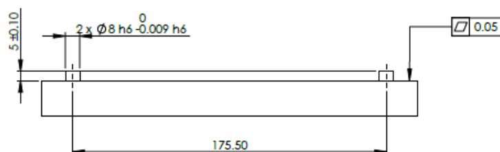
1.2: Mounting plate for Robot base
