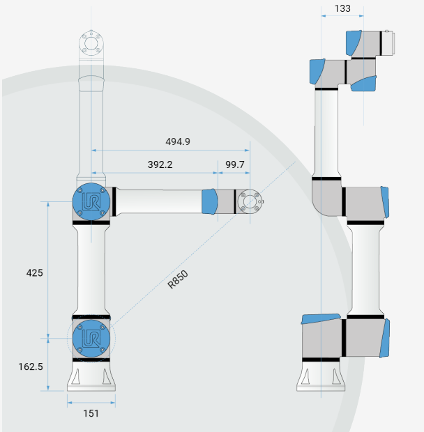
Dimensions and reach of UR7e
