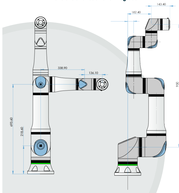
Dimensions and reach of UR18g-950
