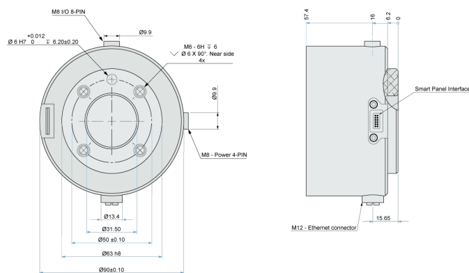
Tool flange for UR18g-950
