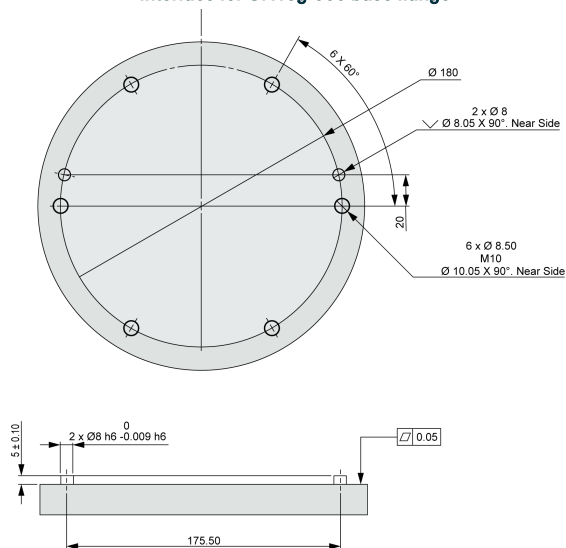
Interface for UR18g-950 base flange
