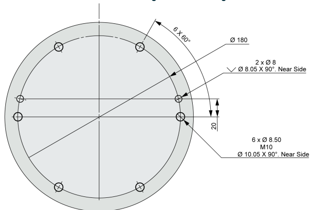
Interface for UR17g-1300 base flange
