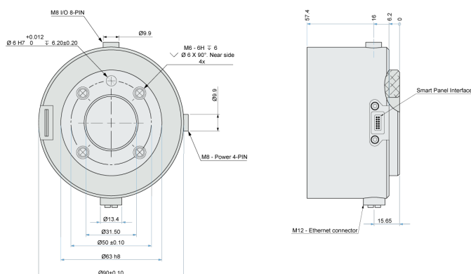
Tool flange for UR17g-1300
