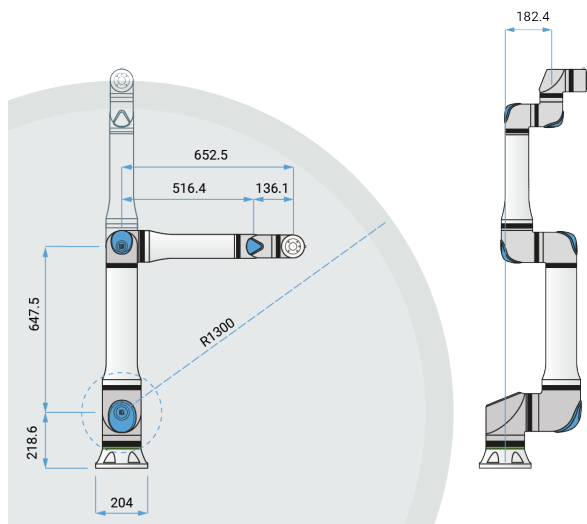
Dimensions and reach of UR17g-1300
