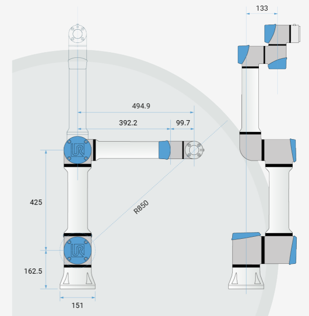
Dimensions and reach of UR7e
