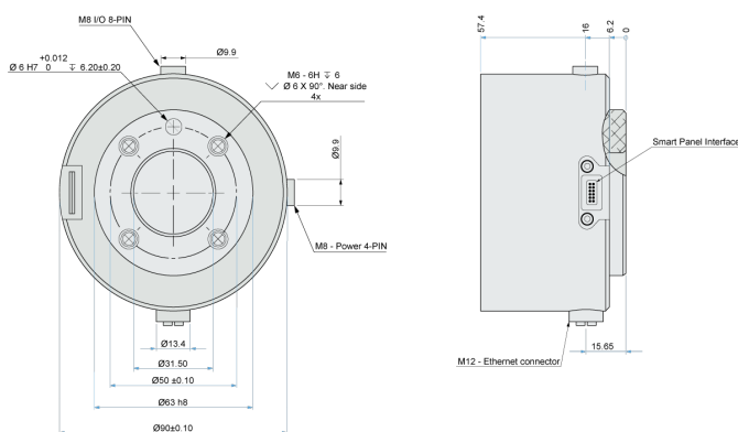
Tool flange for UR17g-1300
