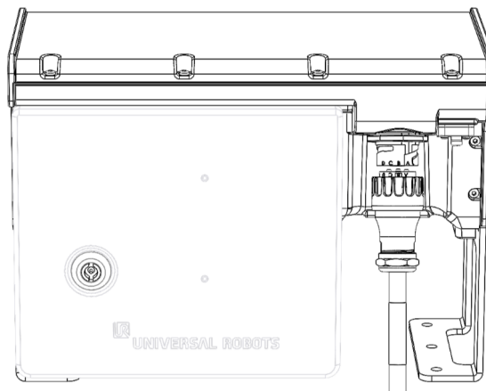
Robot cable connection to Control Box
